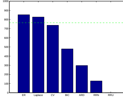
Figure 5: The number of times each estimator picked the correct dimensionality in 1000 replications. ( d = 10, k = 5, N = 100 )
